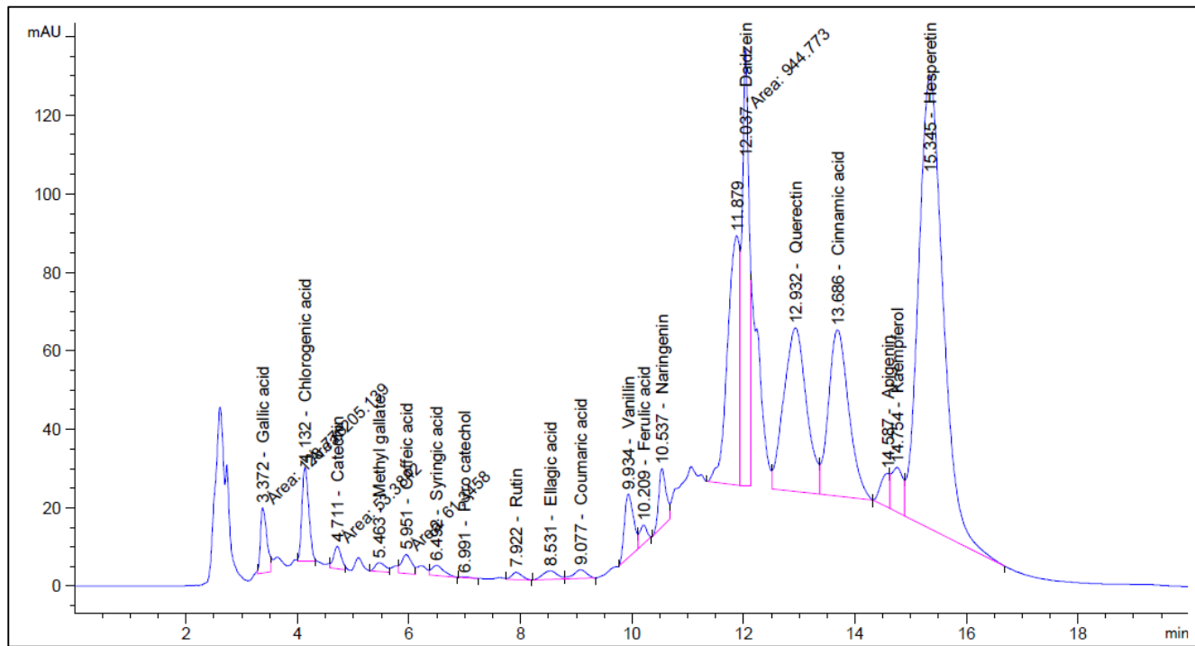
Supplementary Figure 1: HPLC chromatogram of Tribulus terrestris methanol extract, signals at 280 nm.
